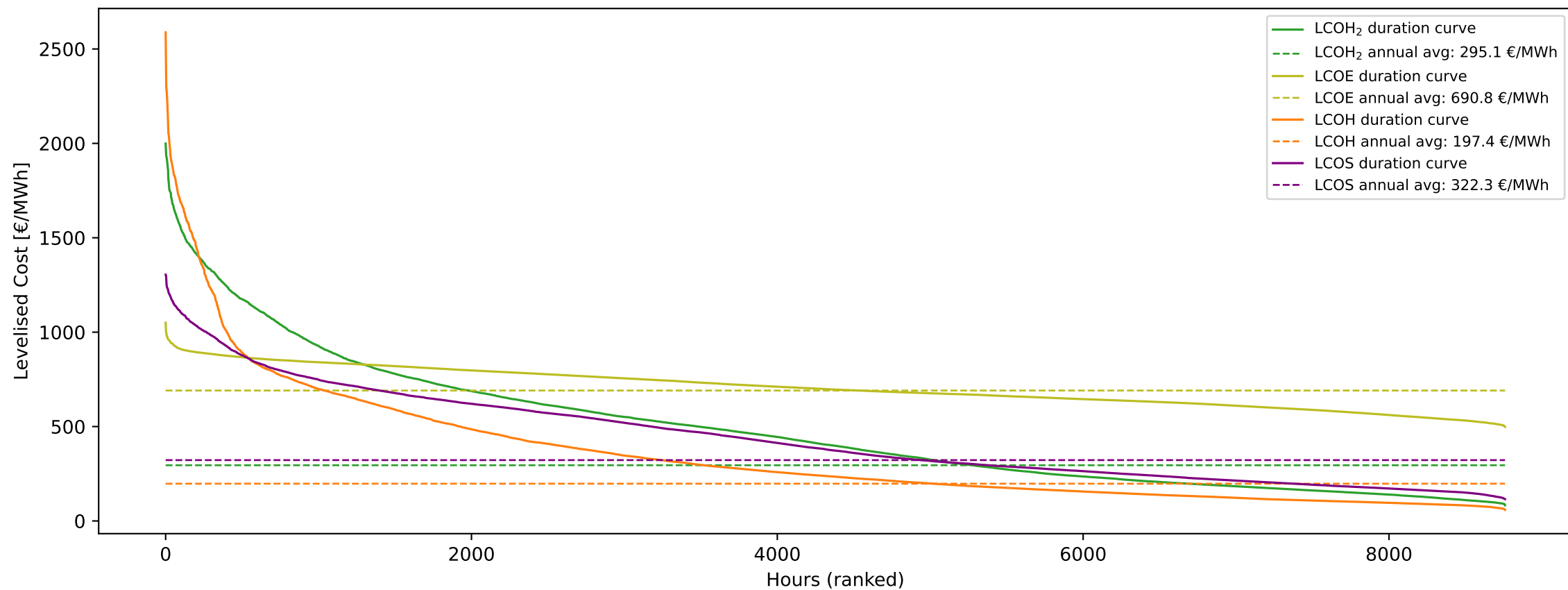
Levelised Cost Duration Curves
